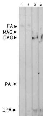
Fig. 2. Assessment of [ ^3\text{H} ]LPA metabolism. Membrane fractions were incubated with [ ^3\text{H} ]LPA (0.5 nM) for 60 min (see Fig. 1). The radioactive membrane lipids were extracted and separated on HPTLC plates (see Section 2). Lane 1 (run in duplicate) shows the methanol/water fraction and lane 2 (duplicate) the chloroform fraction.
